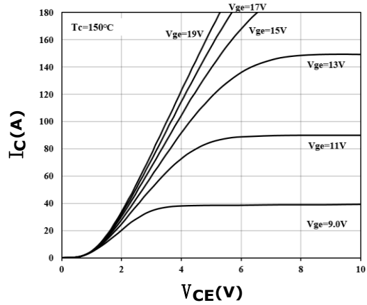
Figure 2. Output Characteristics
