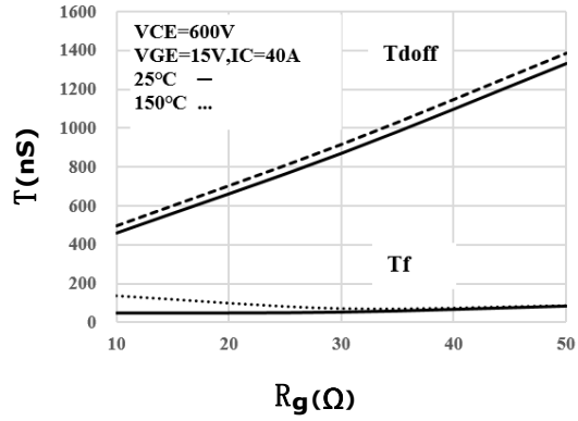
Figure 8. Closing Time-RG Characteristics
