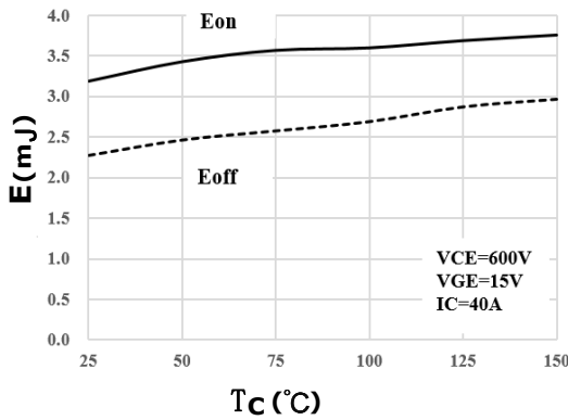
Figure 9. Switching loss-Tc Characteristics
