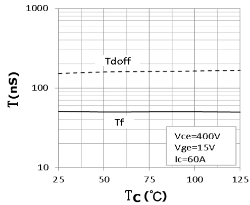
Figure 10. Closing Time-Tc Characteristics
