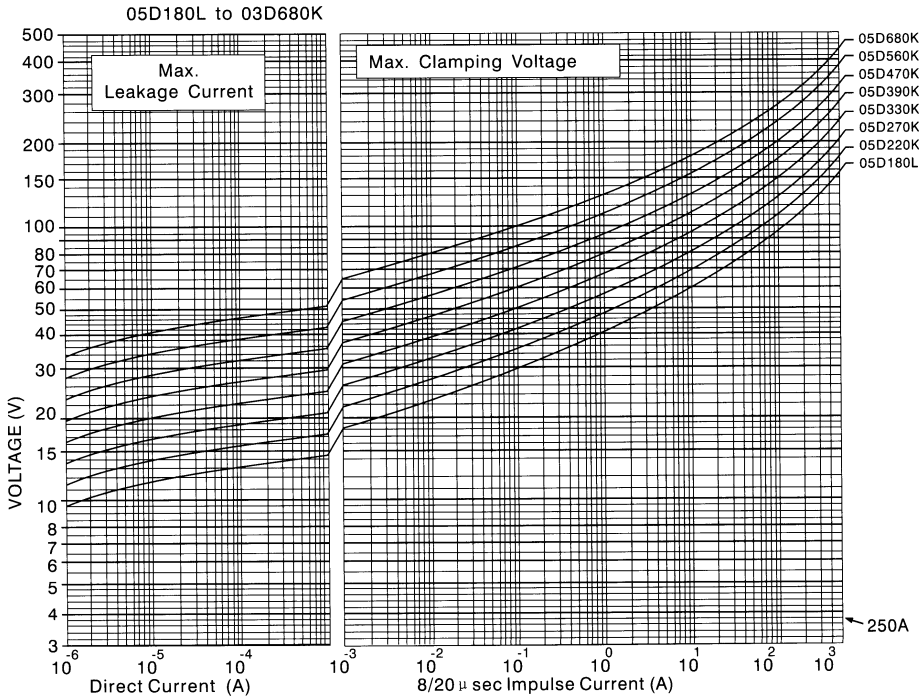
V-I curve
