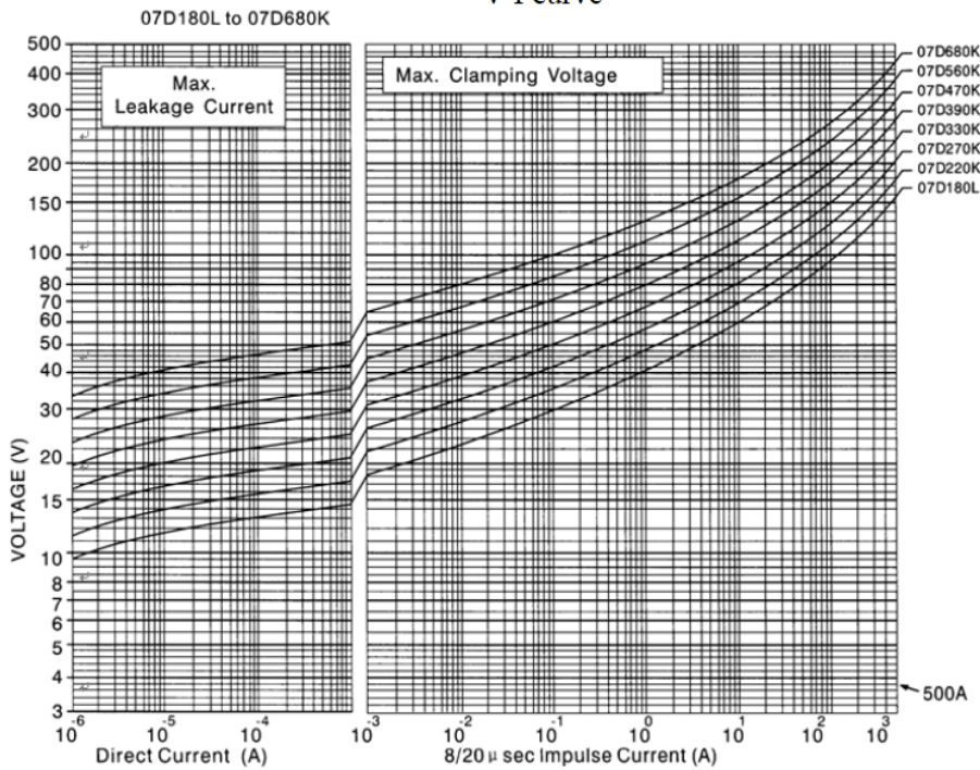
V-I curve
