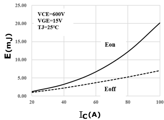
Figure 12. Switching Loss- I_c Characteristics
