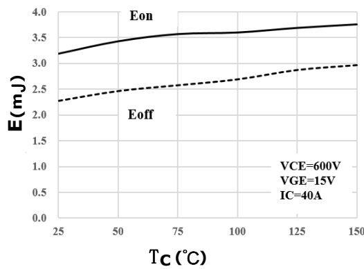
Figure 9. Switching loss- T_c Characteristics
