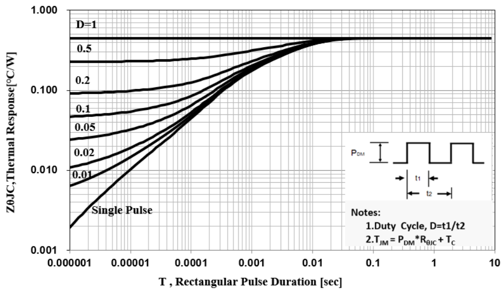
Figure 20. Transient Thermal Impedance
