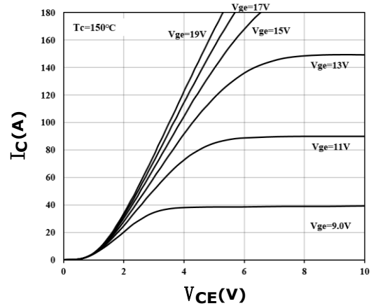
Figure 2. Output Characteristics
