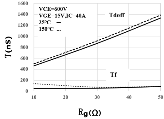
Figure 8. Closing Time- R_g Characteristics
