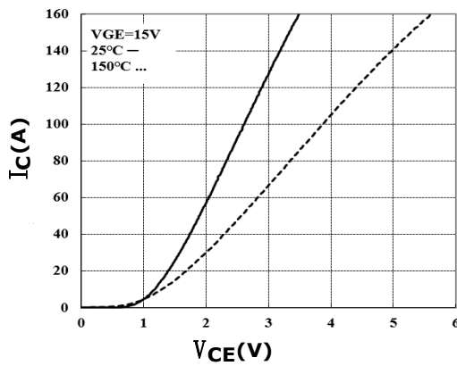
Figure 3. Saturation Voltage Characteristics
