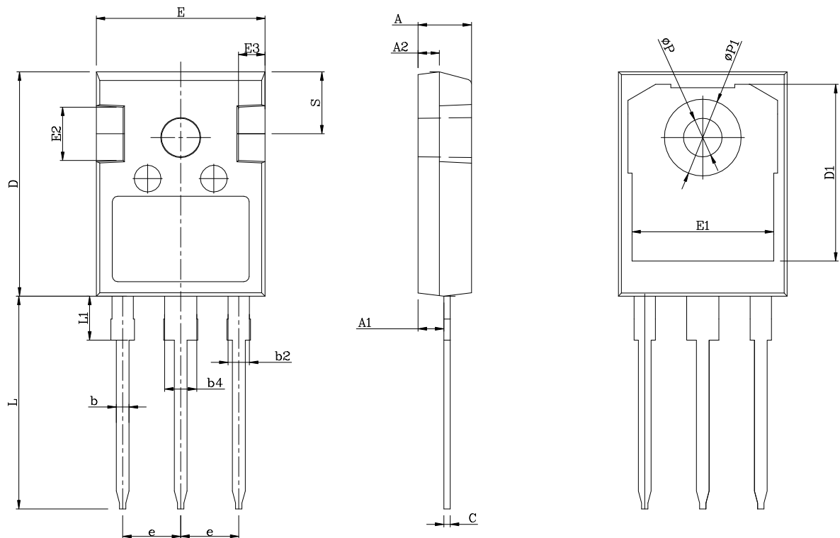
COMMON DIMENSIONS
