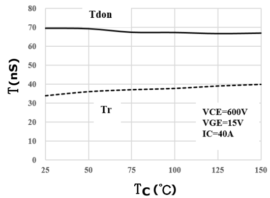
Figure 10. Opening Time- T_c Characteristics
