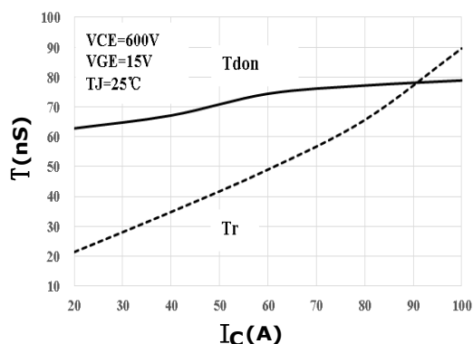
Figure 13. Opening Time- I_C Characteristics
