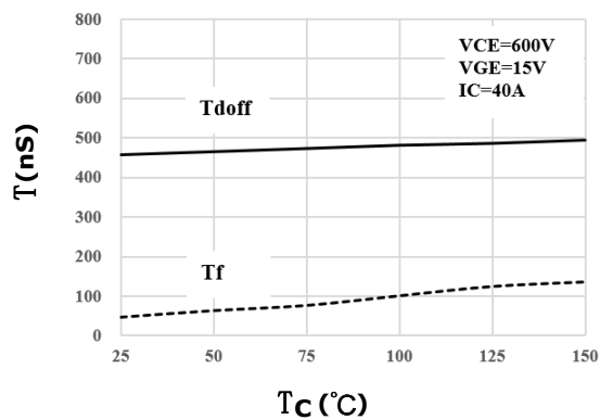
Figure 11. Closing Time- T_c Characteristics
