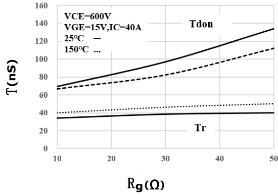
Figure 7. Opening Time- R_g Characteristics
