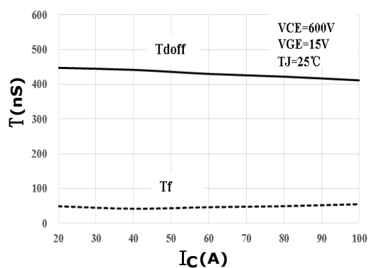
Figure 14. Closing Time- I_C Characteristics
