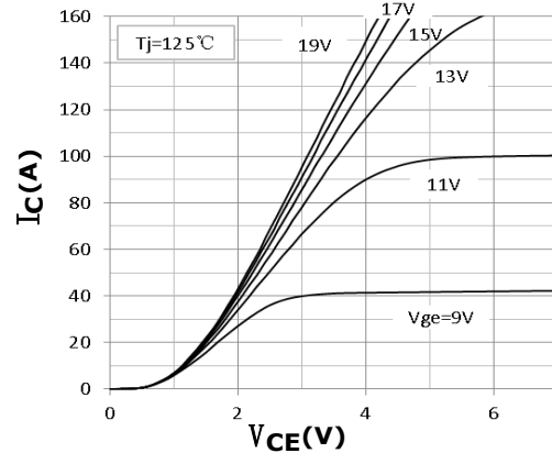
Figure 2. Output Characteristics
