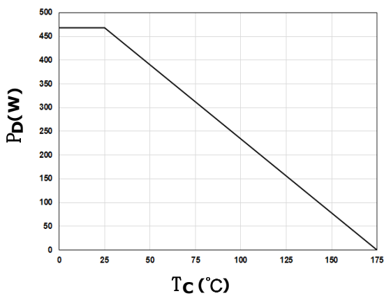
Figure 17. Power Dissipation-Tc Characteristics ( T_J \leq 175^\circ\text{C} )
