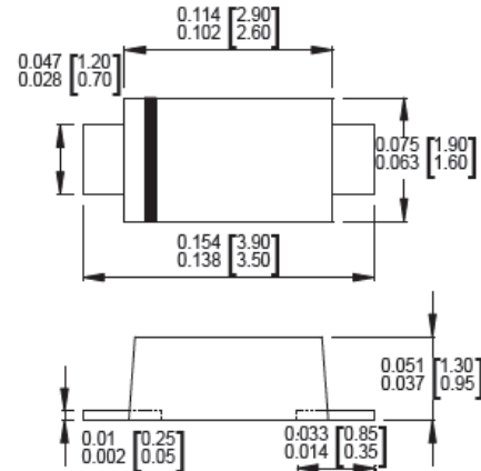
CASE : SOD-123S DIMENSIONS IN INCHES AND (MILLIMETERS)
